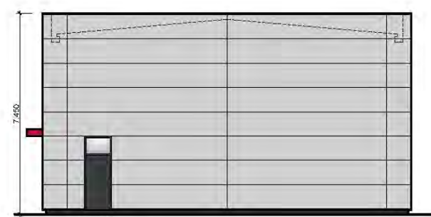
Rear Elevation Fire Exit 7.450
